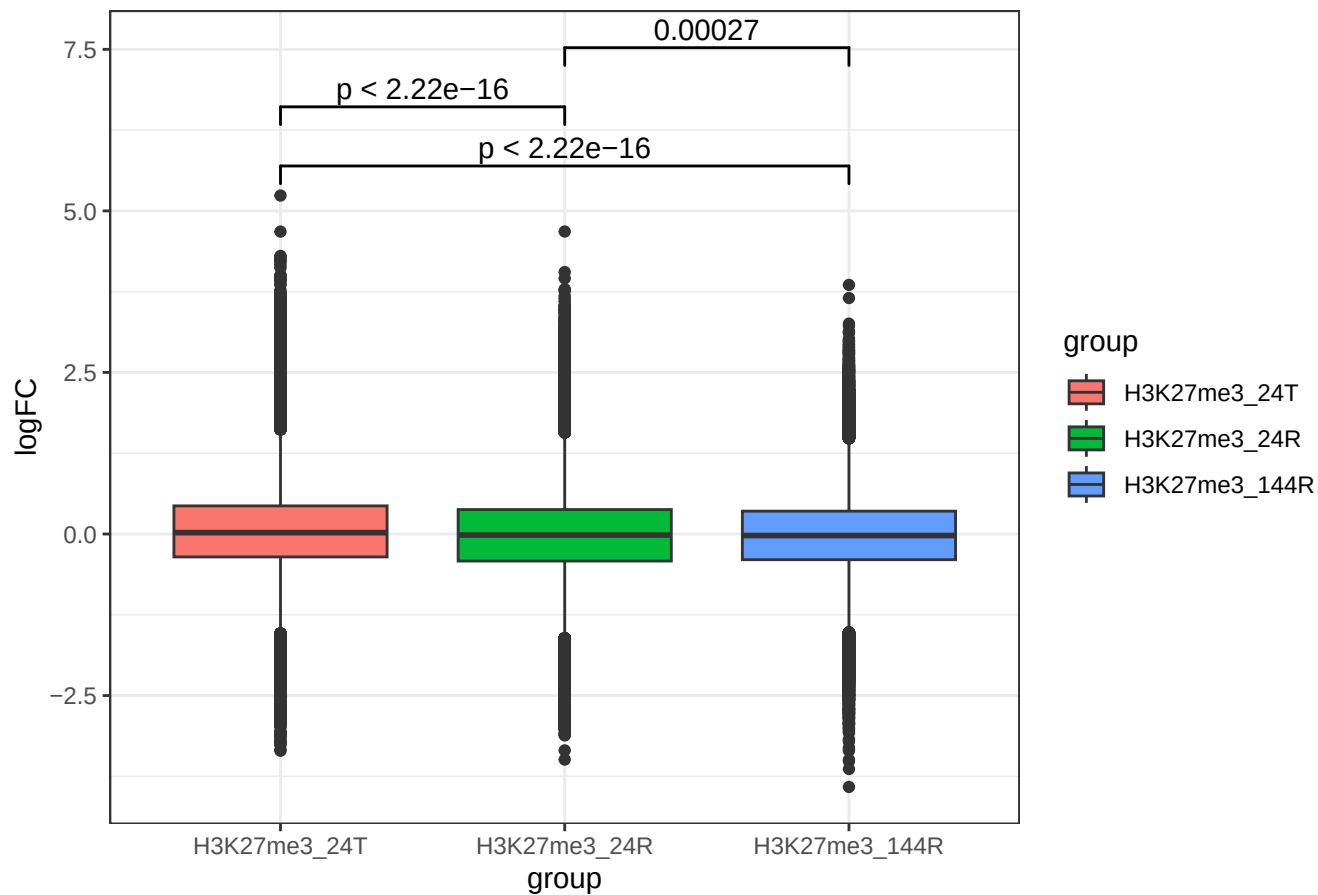
LFC across time for H3K27me3
